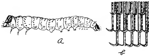
Fig. 458. a, Leopard moth, Zeuzera pyrina L.; b, triordinal crochets.
